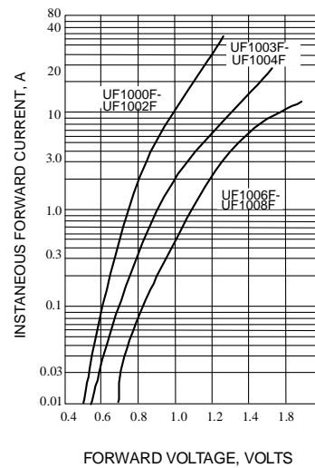
Fig. 5-TYPICAL FORWARD CHARACTERISTICS
