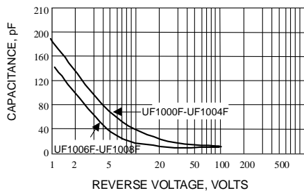
Fig. 4-TYPICAL JUNCTION CAPACITANCE
