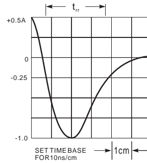
Fig. 1-REVERSE RECOVERY TIME CHARACTERISTIC AND TEST CIRCUIT DIAGRAM
