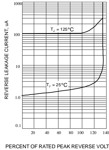
Fig. 2-TYPICAL REVERSE CHARACTERISTICS
