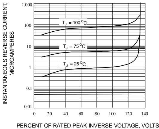
Fig. 3-TYPICAL REVERSE CHARACTERISTICS
