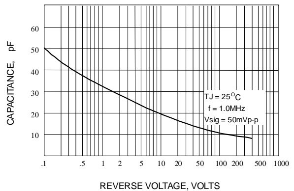
Fig. 6-TYPICAL JUNCTION CAPACITANCE
